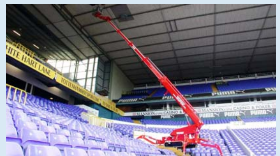
The automatic outrigger system levels out height differences perfectly. Additionally, three different outrigger setup positions are available.
